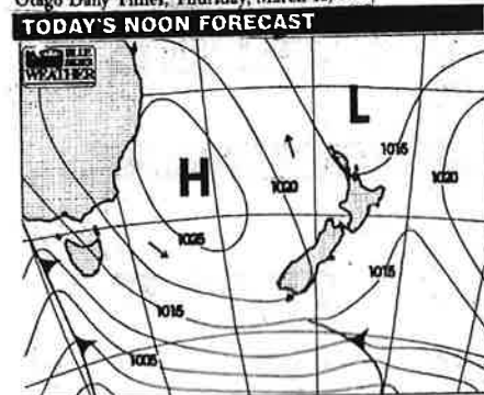
Figure 3. Weather maps of the anticyclone conditions used for the second flight on March 12, to the Fiordland glaciers.
