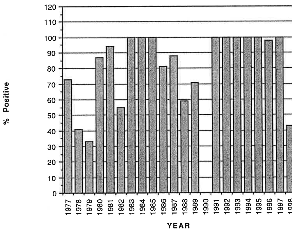
Figure 7. The percentage of all glaciers measured each year showing a positive balance.
