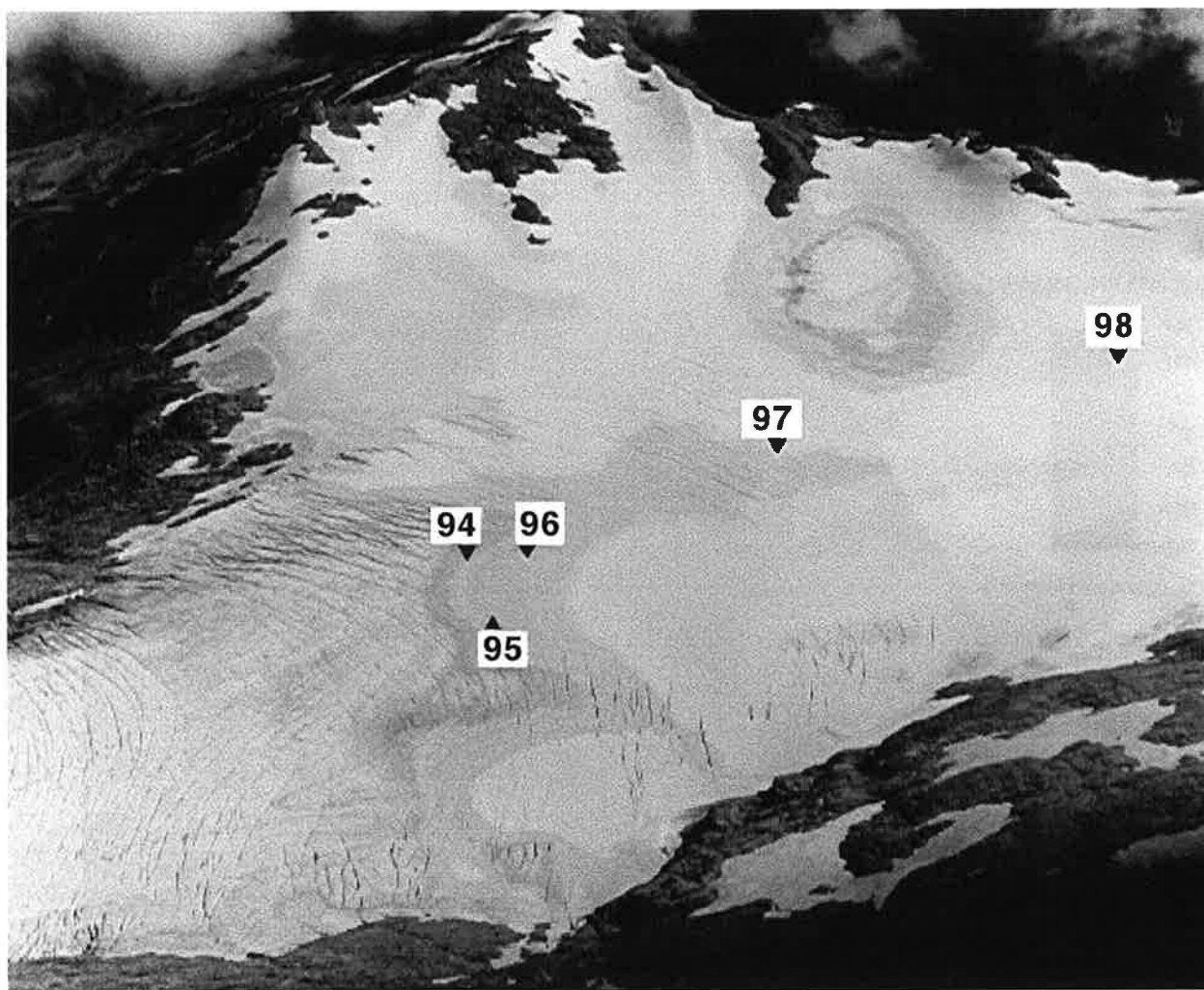
Figure 8. The subtle, high March 1998 snow line and multiple firn lines on Brewster Glacier. Note that the numbers give the year of the ELA measurement , not the year of the snowpack, since the snow fell in the winter of the previous calendar year.
