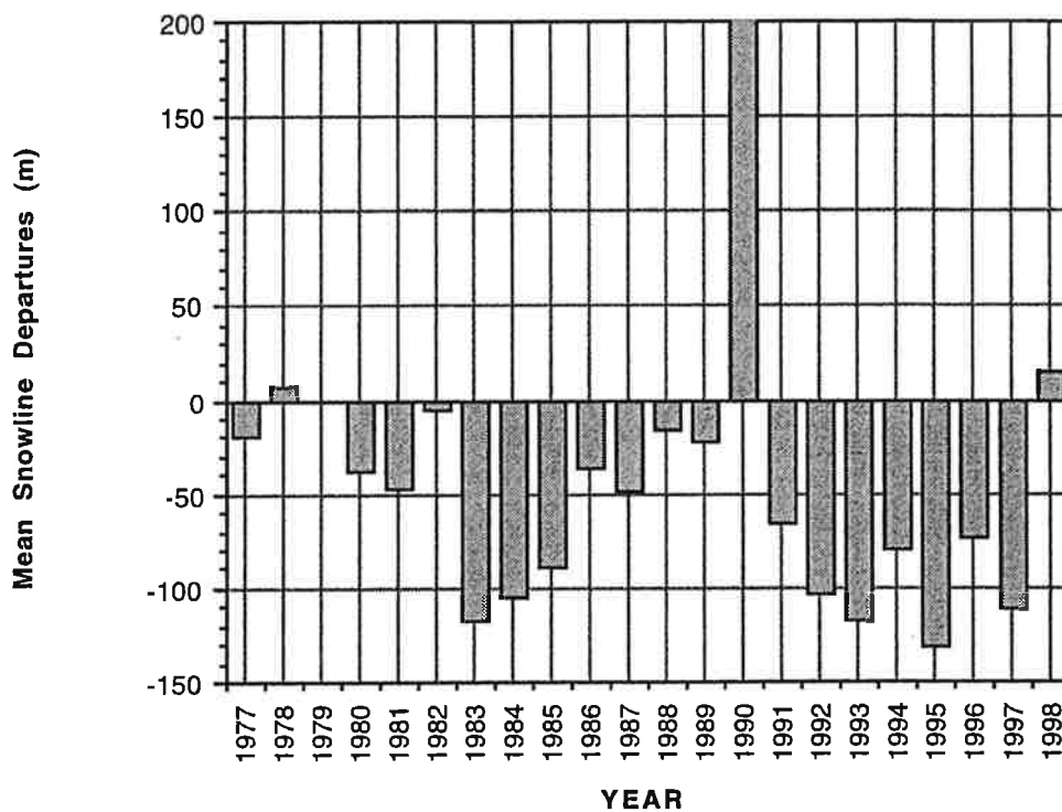
Figure 6. Mean annual snowline elevation departures from the steady-state ELA, for the 21 years, 1977 to 1998.
