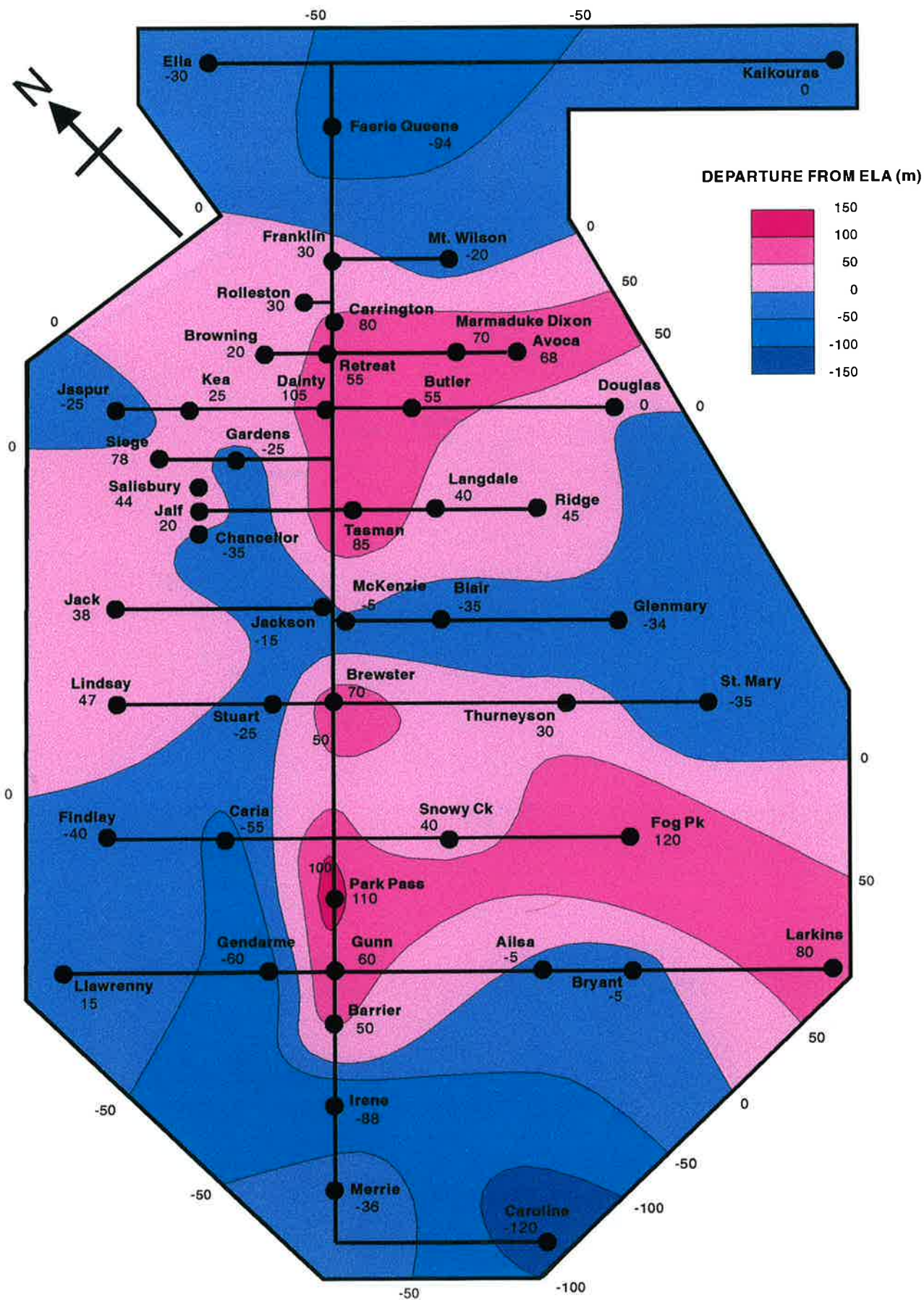
Figure 9. Diagrammatic trend surface for 1998, of departures from the long-term ELA (m)
