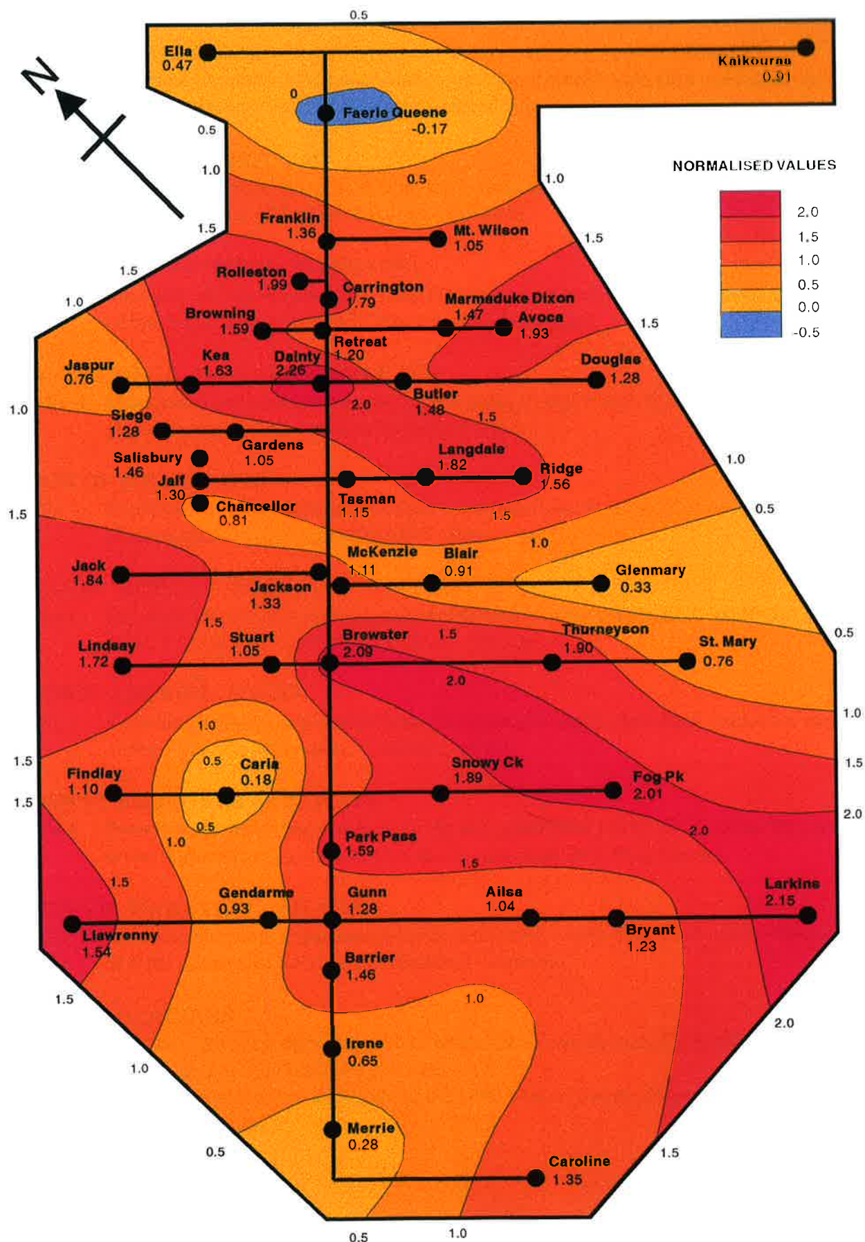
Figure 10. Normalised values for each glacier, plotted as the trend surface for 1998, depicting 1998 departures from the mean record.
