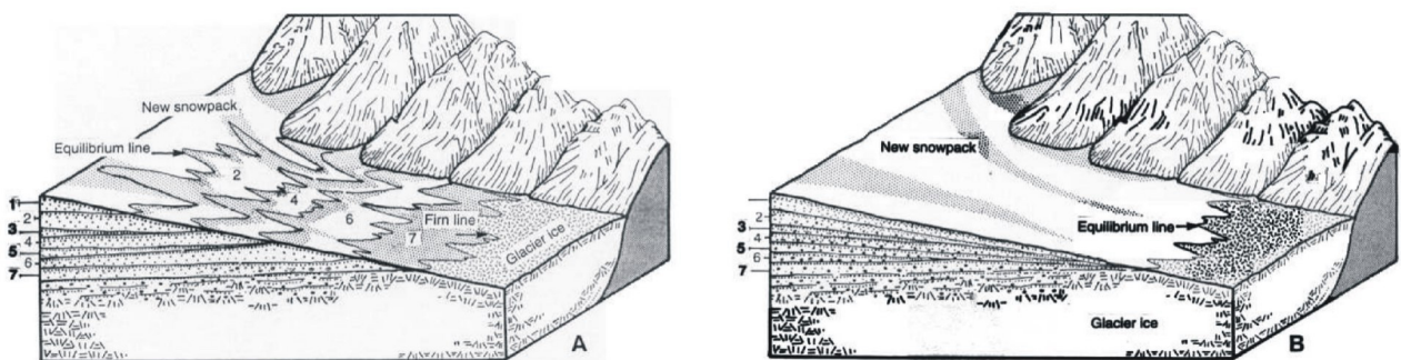
Figure 4 Schematic diagrams of stratigraphy at the glacier equilibrium line. (A) for a year of negative balance (high ELA) and (B) for a year of positive balance (low ELA). Numbers indicate age in years of past firn layers.
