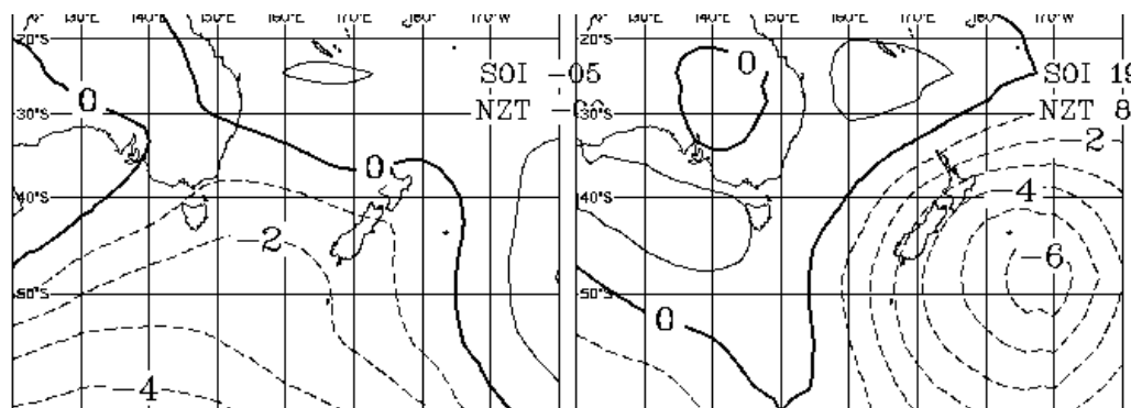
Figure 7. Mean sea level pressure anomalies (a) January – July 2004 and (b) August – December 2004.
