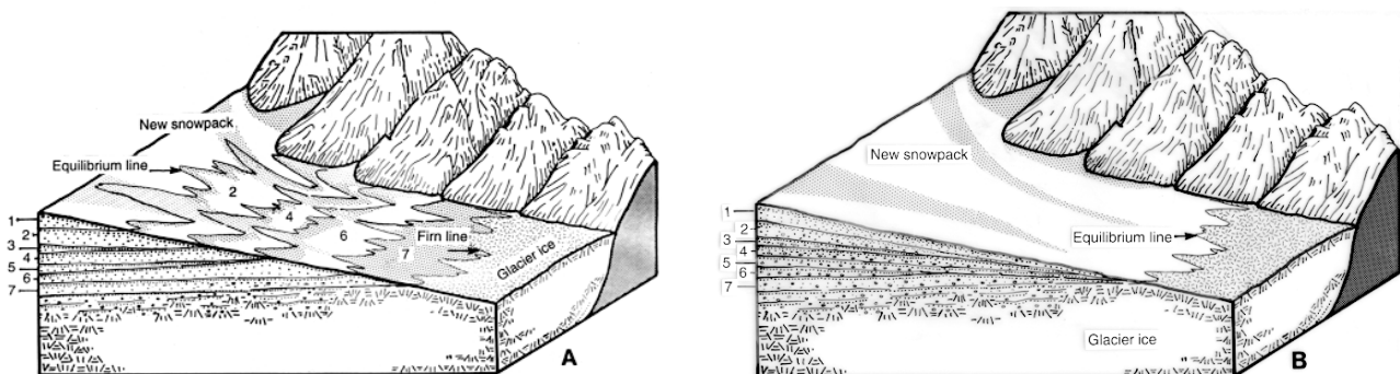
Figure 5: Schematic diagrams of stratigraphy at the glacier equilibrium line. (A) for a year of negative balance (high ELA) and (B) for a year of positive balance (low ELA). Numbers indicate age in years of past firn layers.
