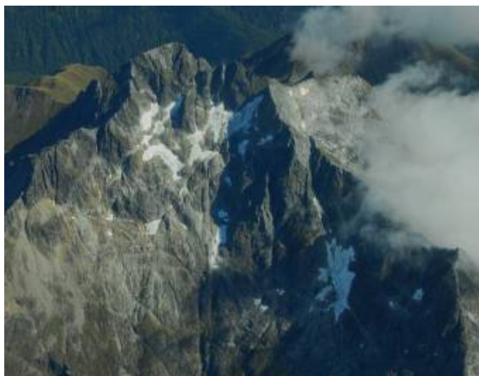
Photograph 55: Caroline Peak on 12 March 2011, resolution reduced to 200dpi.
