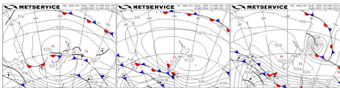
Figure 2-2: Weather maps for Flight on 12 March (left) and 13 March 2011 (middle), and flight two on 30 March (right). Courtesy of Ross Marsden, MetService New Zealand.
