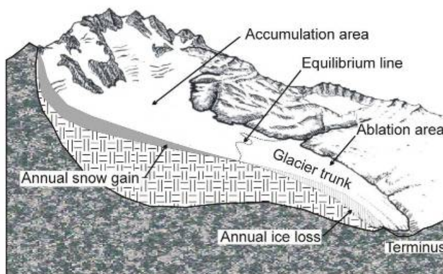
Figure 1-2: Basic parameters of a glacier.
