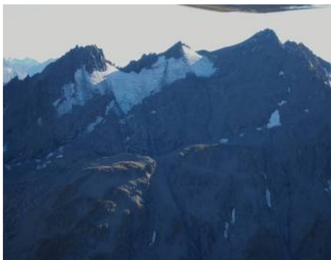
Photograph 43: Mt Larkins on 30 March 2011, resolution reduced to 200dpi.
