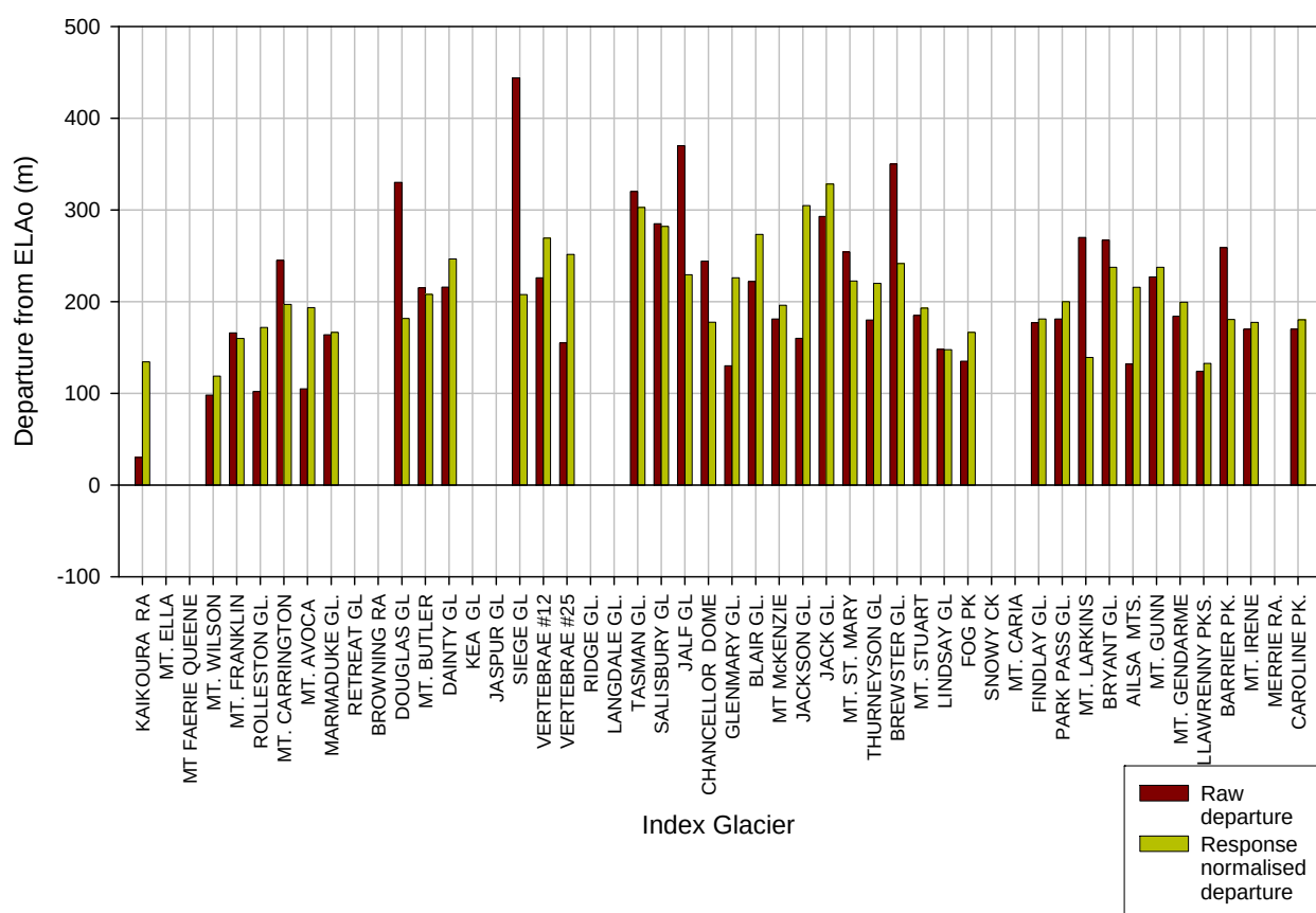
Figure 4-1: Histogram plot giving the 2010/2011 snowline departures (raw and response normalised) for each index glacier from the long-term ELAo.
