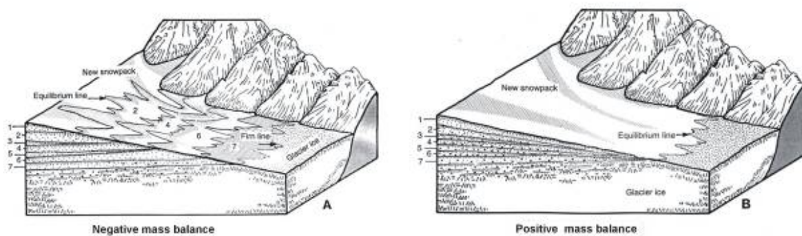
Figure 3-1: Schematic diagrams of stratigraphy at the glacier equilibrium line. (A) for a year of negative balance (high ELA) and (B) for a year of positive balance (low ELA). Numbers indicate age in years of past firm layers.
