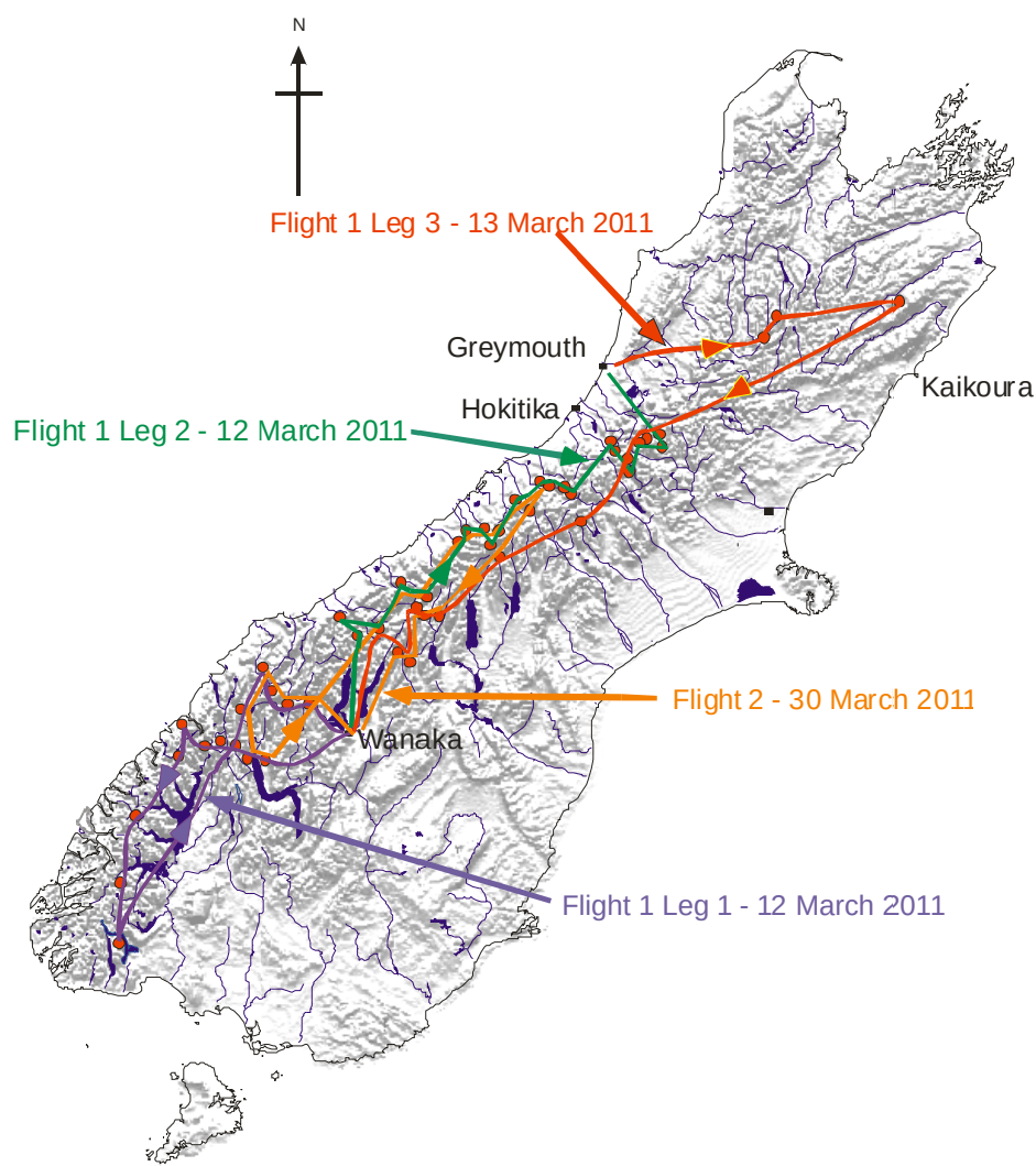
Figure 2-1: Flight paths for the two flights of the 2011 glacier survey. Flight one completed on 12 and 13 March, and flight two on 30 March.
