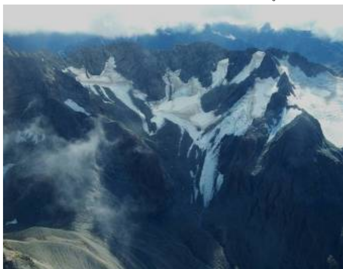
Photograph 9: Marmaduke Dixon 12 March 2011, resolution reduced to 200dpi.
