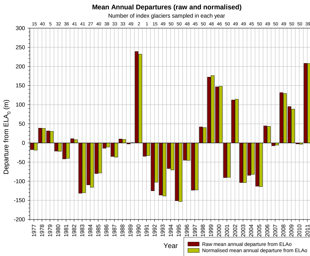
Figure 4-2: Mean annual departures (raw and normalised) from the ELAo for all measured glaciers for the entire period of these surveys.
