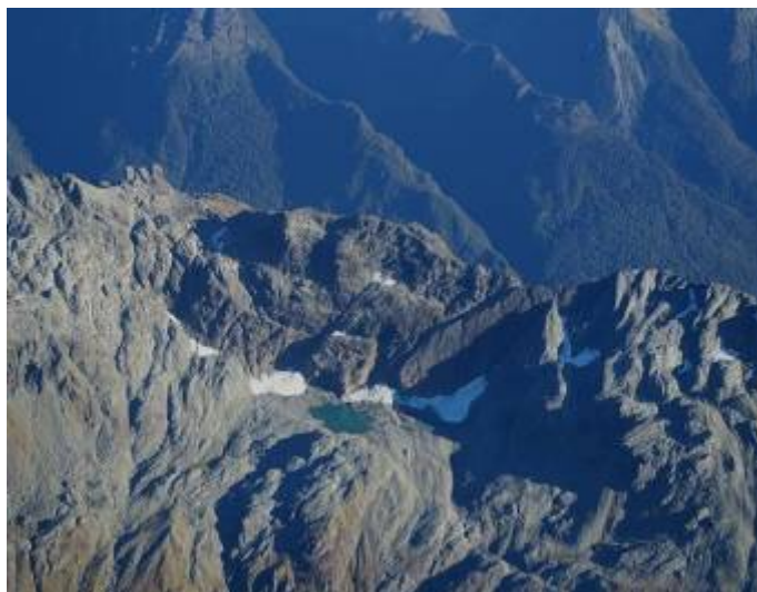
Photograph 38: Mt Caria on 30 March 2011, resolution reduced to 200dpi.
