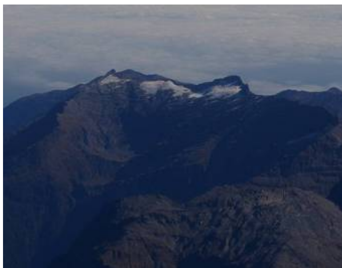
Photograph 35: Lindsay Glacier on 30 March 2011, resolution reduced to 200dpi.
