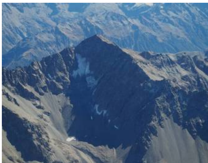
Photograph 31: Mt St Mary on 30 March 2011, resolution reduced to 200dpi.
