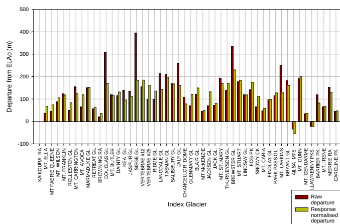
Figure 4-1: Histogram plot giving the 2011/2012 snowline departures (raw and response normalised) for each index glacier from the long-term ELAo.
