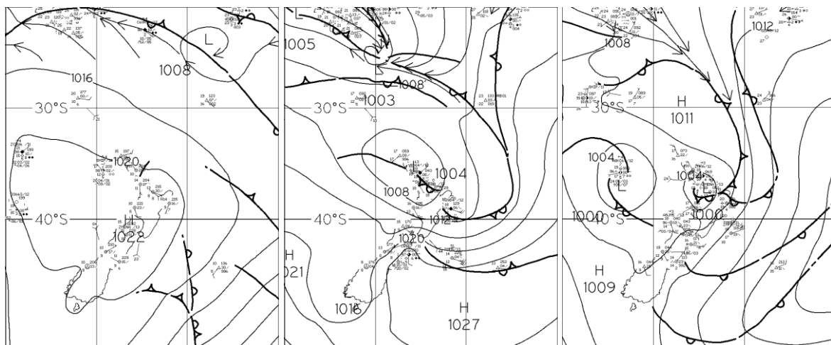
Figure 2-2: Barometric pressure charts for Flight one on 4 March 2012 (left), Flight two on 20 March (centre), and 21 March (right). Courtesy of MetService New Zealand.
