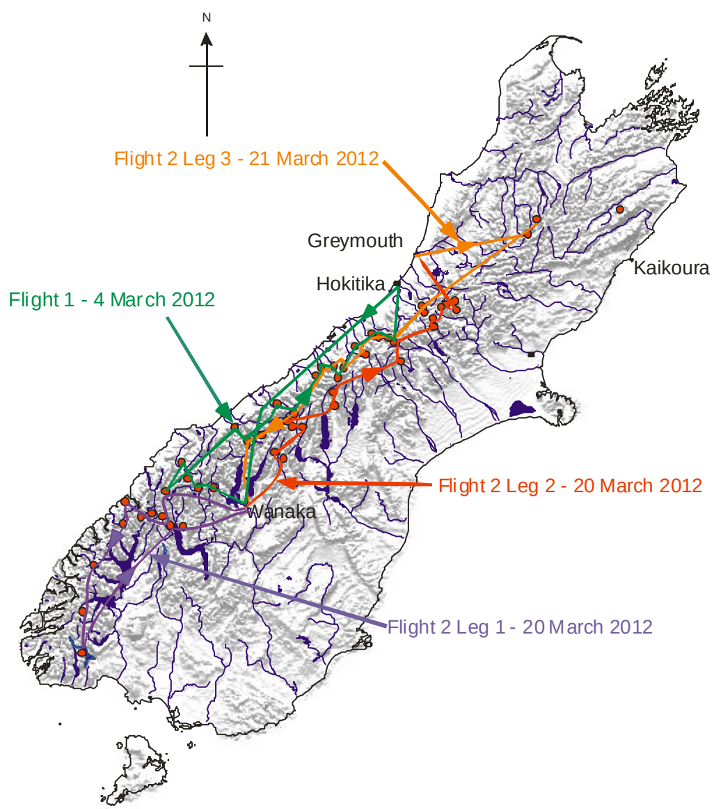
Figure 2-1: Flight paths for the two flights of the 2012 glacier survey. Flight one completed on 4 March, and flight two on 20 and 21 March.
