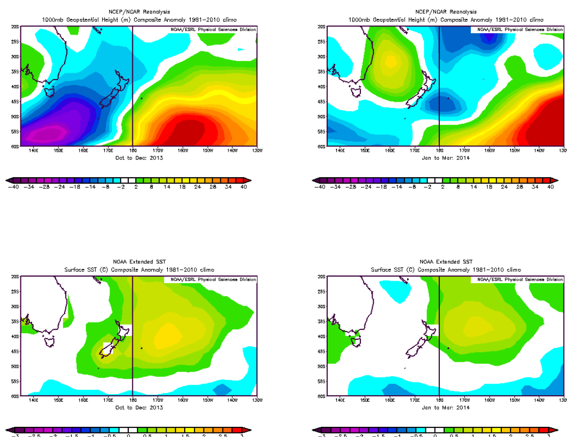
Figure 4-2: Southwest Pacific anomalies at the 1000hPa geopotential height (top row) October-December 2013 (left) and January-March 2014 (right). See Figure 4-3 for details about contours.
