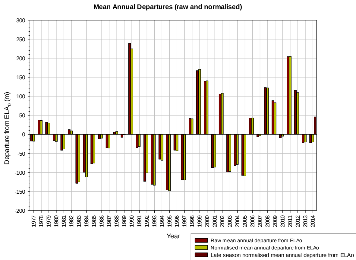
Figure 4-5: Mean annual departures (raw and normalised) from the ELA₀ for all measured glaciers for the entire period of the surveys.
