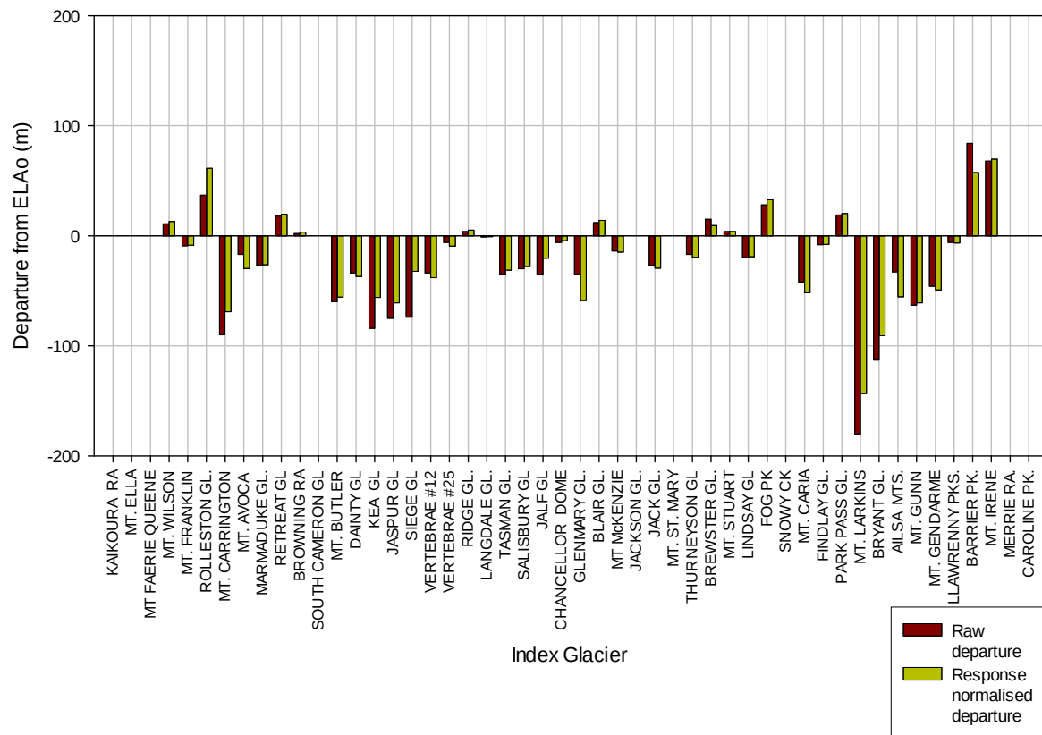
Figure 4-3: Histogram plot of the 2013/2014 snowline departures (raw and response normalised) for each index glacier from the long-term ELAo.
