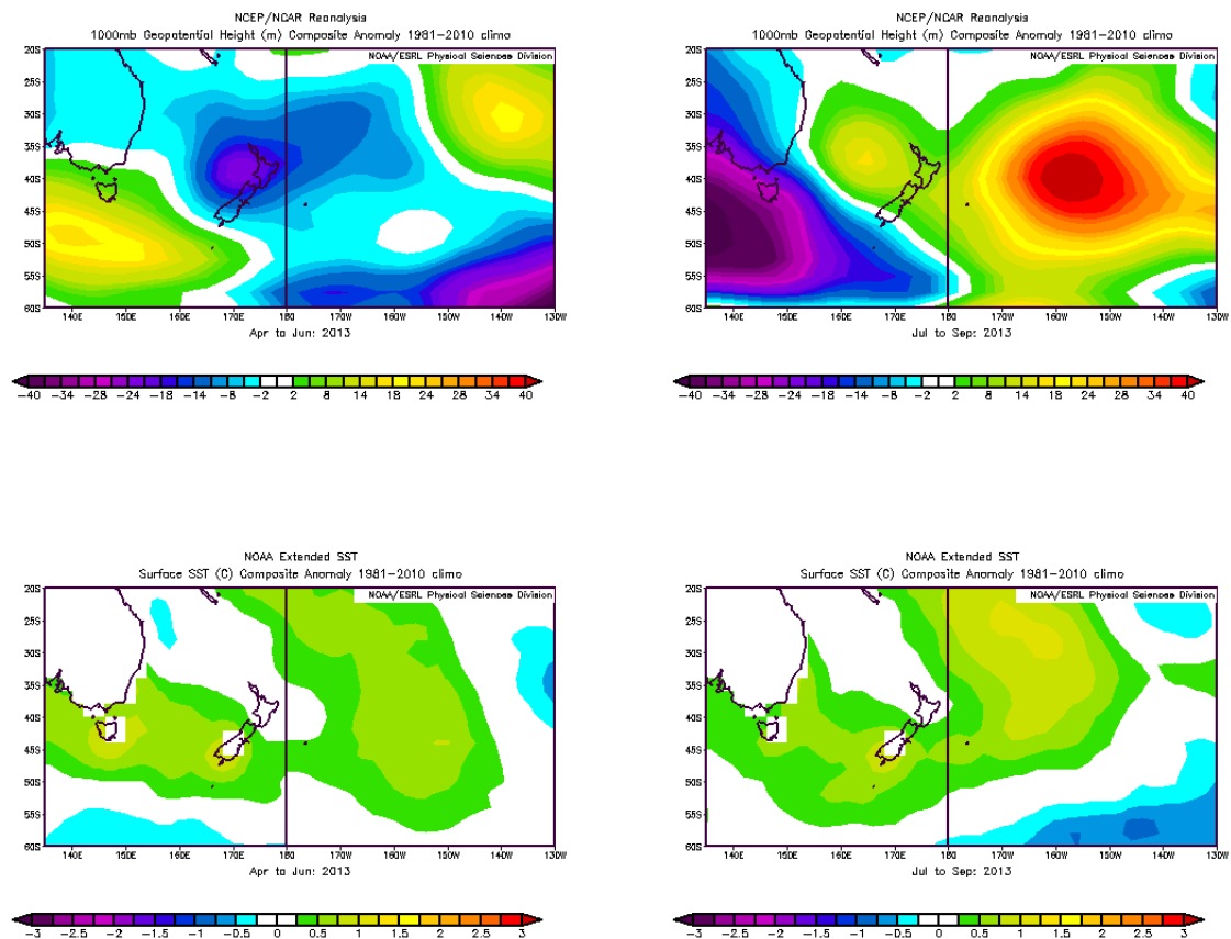
Figure 4-1: Southwest Pacific anomalies at the 1000hPa geopotential height (top row) April-June 2013 (left) and July-September 2013 (right). Geopotential indicates areas of relatively high or low pressure (green/red shades indicating 'highs', blue/purple shades indicating 'lows'). The bottom row shows the corresponding sea surface temperature (SST) anomalies across the New Zealand sector for the same time period (green/red shades indicating warmth, blue/purple shades indicating cool).
