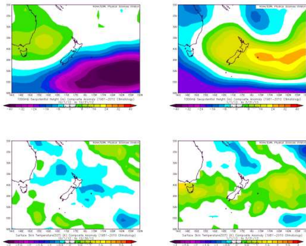
Figure 4-2: Southwest Pacific anomalies at the 1000hPa geopotential height (top row) October-December 2012 (left) and January-March 2013 (right). See Figure 4-3 for details about contours.
