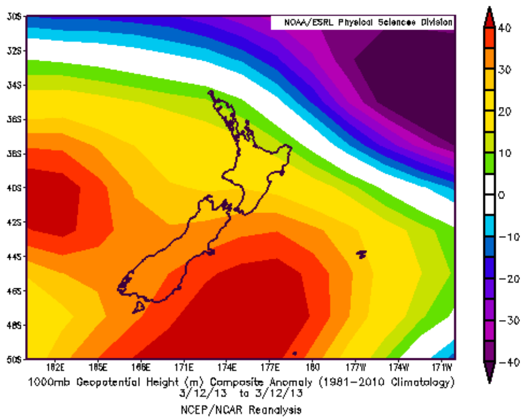
Figure 2-2: Geopotential height anomaly map at the 1000hPa level for the flight on 12 March 2013. Courtesy of NCEP/NCAR reanalysis. Anomalies are relative to the 1981-2010 average conditions.
