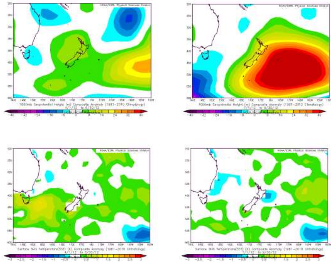
Figure 4-1: Southwest Pacific anomalies at the 1000hPa geopotential height (top row) April-June 2012 (left) and July-September 2012 (right). Geopotential indicates areas of relatively high or low pressure (green/red shades indicating 'highs', blue/purple shades indicating 'lows'). The bottom row shows the corresponding sea surface temperature (SST) anomalies across the New Zealand sector for the same time period (green/red shades indicating warmth, blue/purple shades indicating cool).
