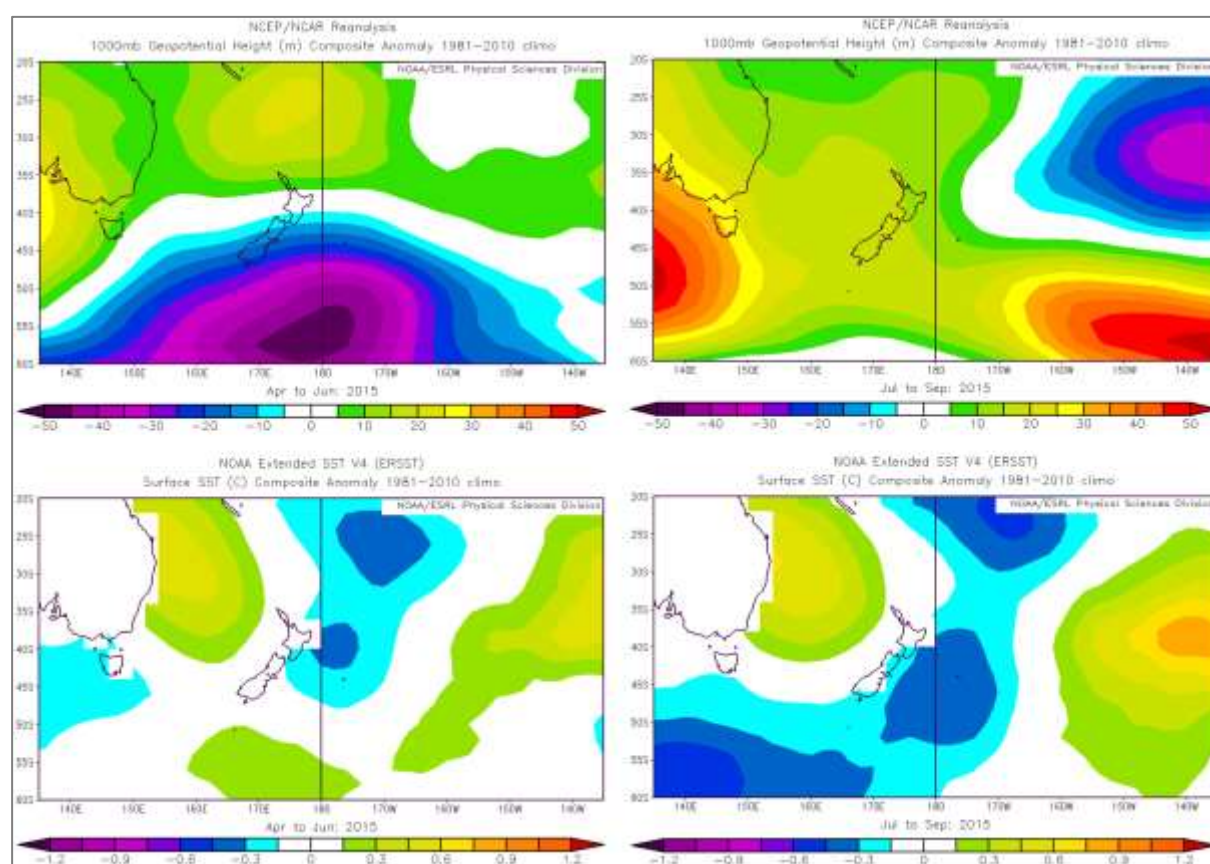
Figure 4-1: Southwest Pacific anomalies at the 1000hPa geopotential height (top row) April-June 2015 (left) and July-September 2015 (right). Geopotential indicates areas of relatively high or low pressure (green/red shades indicating 'highs', blue/purple shades indicating 'lows'). The bottom row shows the corresponding sea surface temperature (SST) anomalies across the New Zealand sector for the same time period (green/red shades indicating warmth, blue/purple shades indicating cool).
