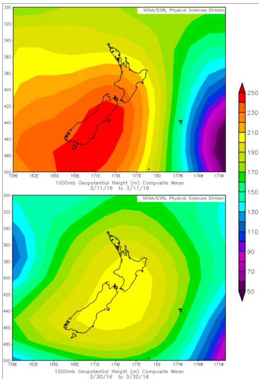
Figure 2-2: Geopotential height maps at the 1000hPa level for the flights on 11 March 2016 (top) and 30 March 2016 (bottom). Courtesy of NCEP/NCAR reanalysis.
