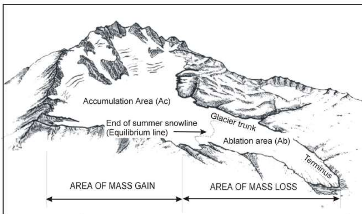
Figure 4: Basic parameters of a glacier.
