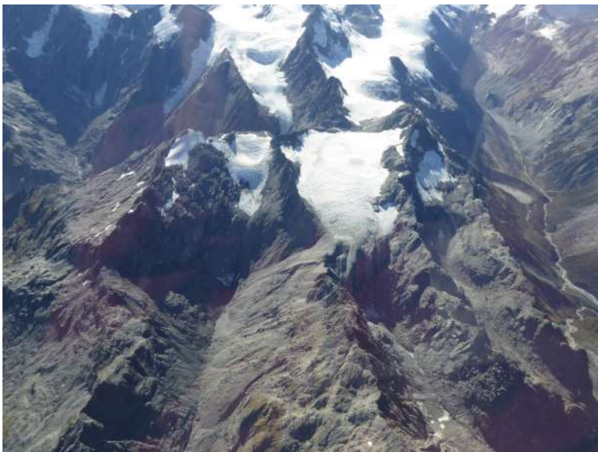
Figure D-17: Vertebrae Glacier 25 (right) on 11 March 2018.
