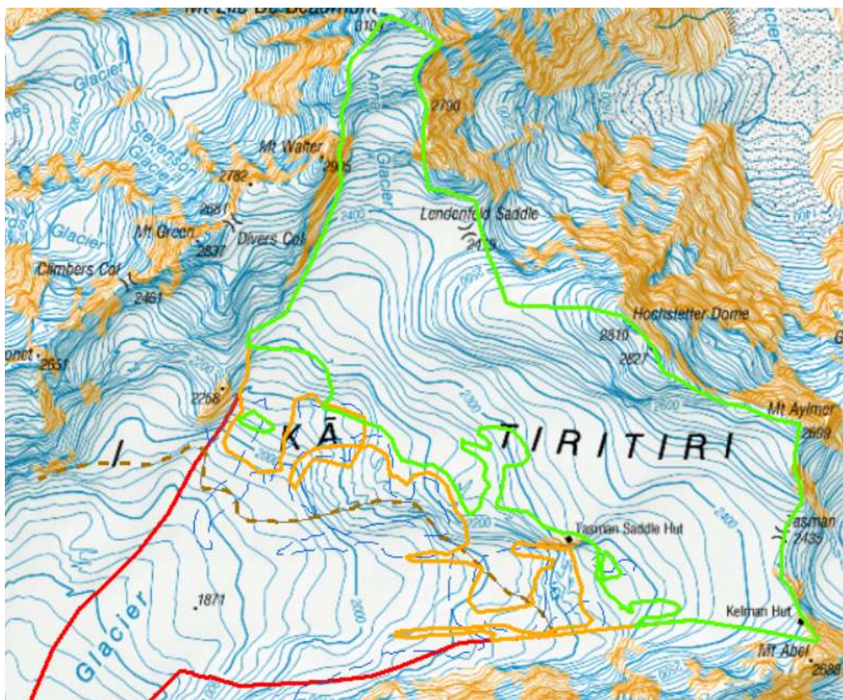
Figure E-3: Mapped Tasman snowline elevations for 1990 (brown dashed), 2018 (orange solid), and 2019 (green solid).
