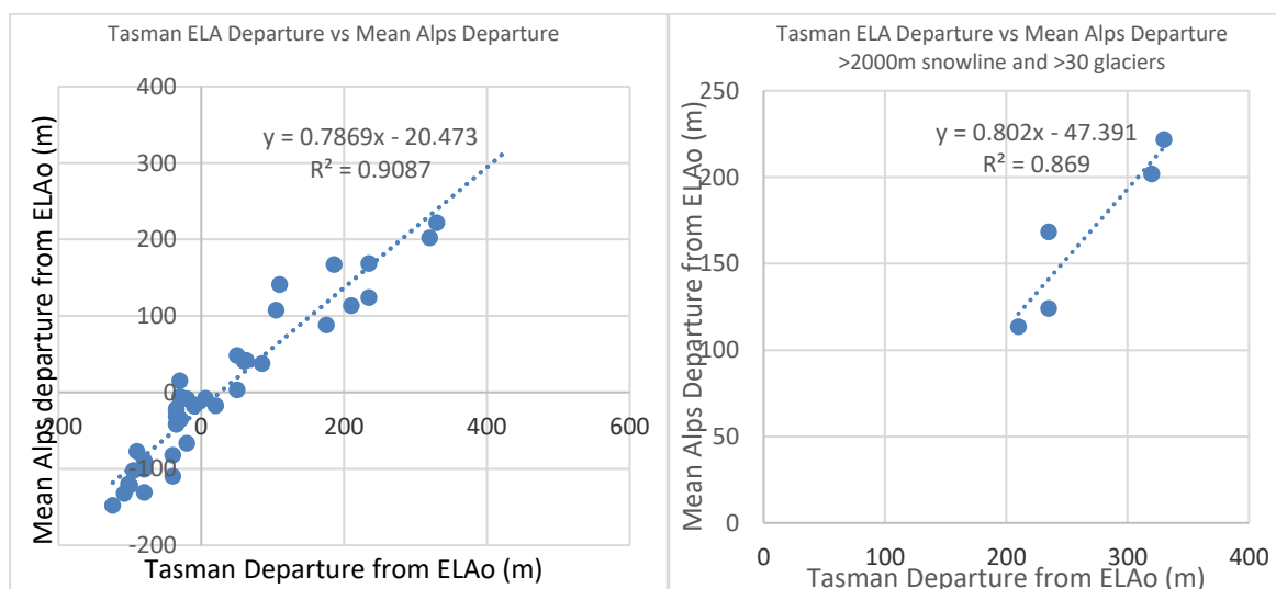
Figure E-4: Regression between all Tasman ELA departures and the mean Alps departures (left), and Tasman ELAs vs mean Alps departures where >30 observations in the year and Tasman snowline >2000m (right).
