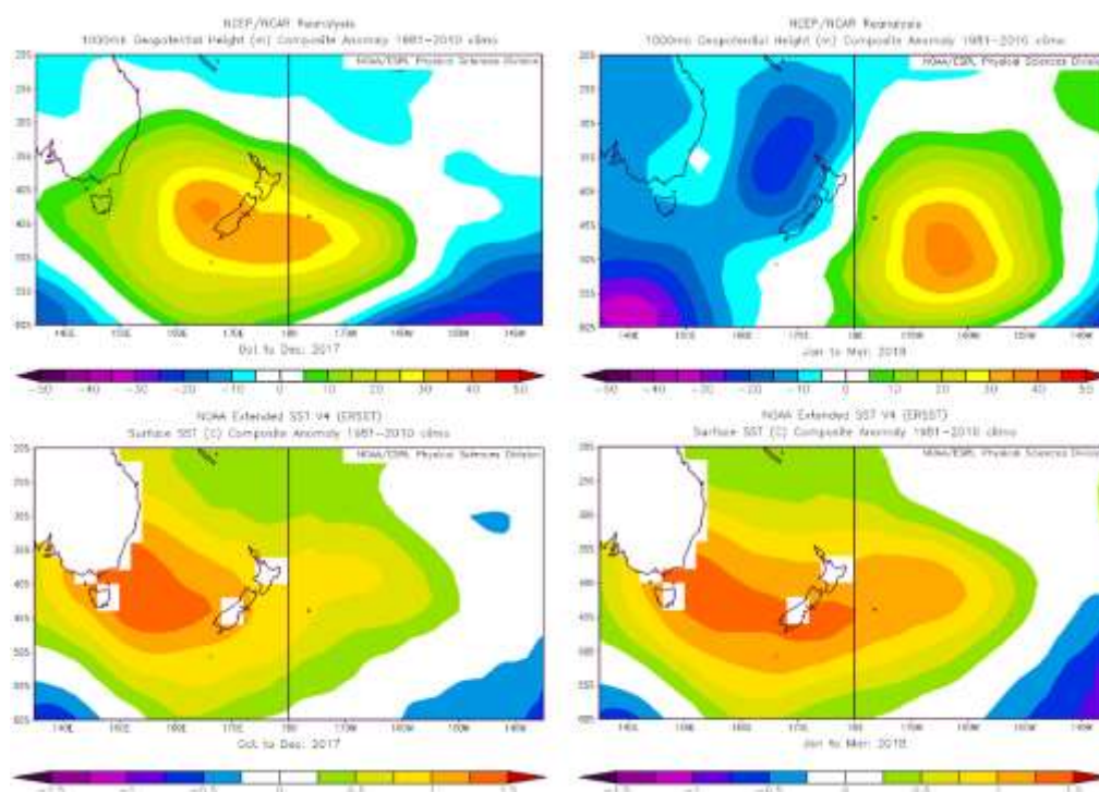
Figure 6: Southwest Pacific anomalies at the 1000hPa geopotential height (top row) October-December 2017 (left) and January-March 2018 (right). The bottom row shows the corresponding sea surface temperature (SST) anomalies across the New Zealand sector for the same time.
