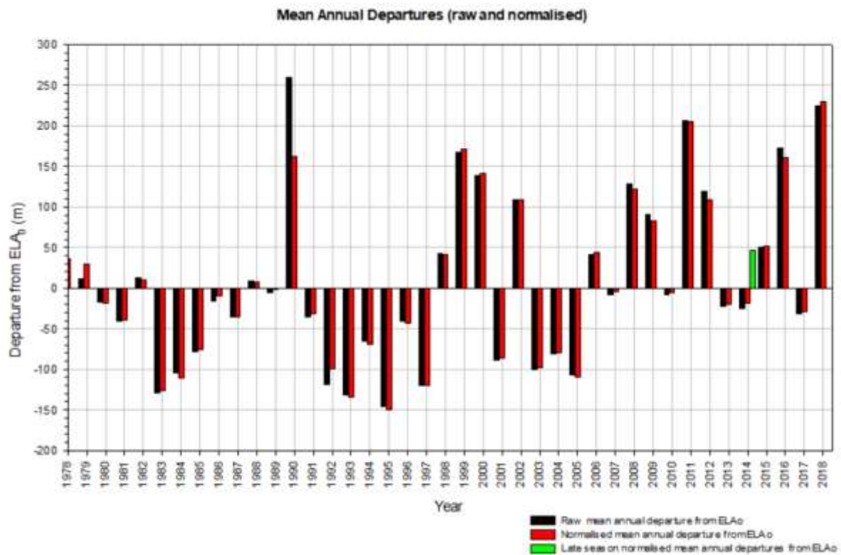
Figure 8: Mean annual departures (raw and normalised) from the ELA0 for all measured glaciers for the entire period of the surveys.
