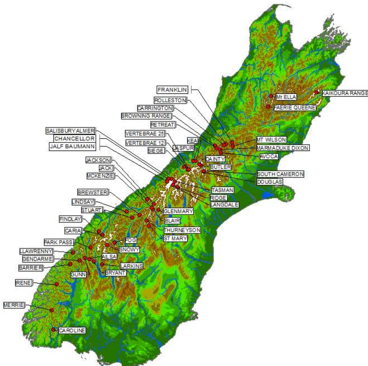
Figure 1: Location of the 50 index glaciers across the South Island of New Zealand.
