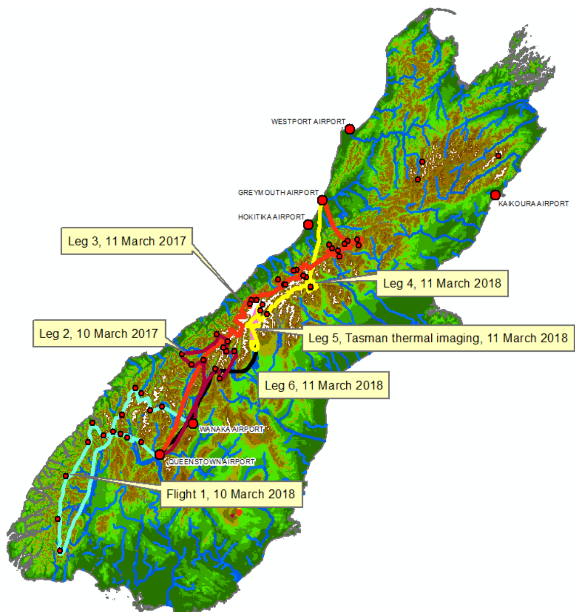
Figure 3: An overview of the glacier flight path for 2018.
