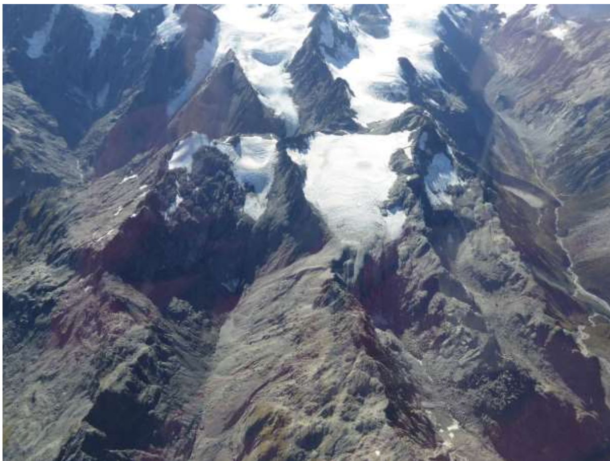
Figure D-16: Vertebrae 12 Glacier (left) on 11 March 2018.
