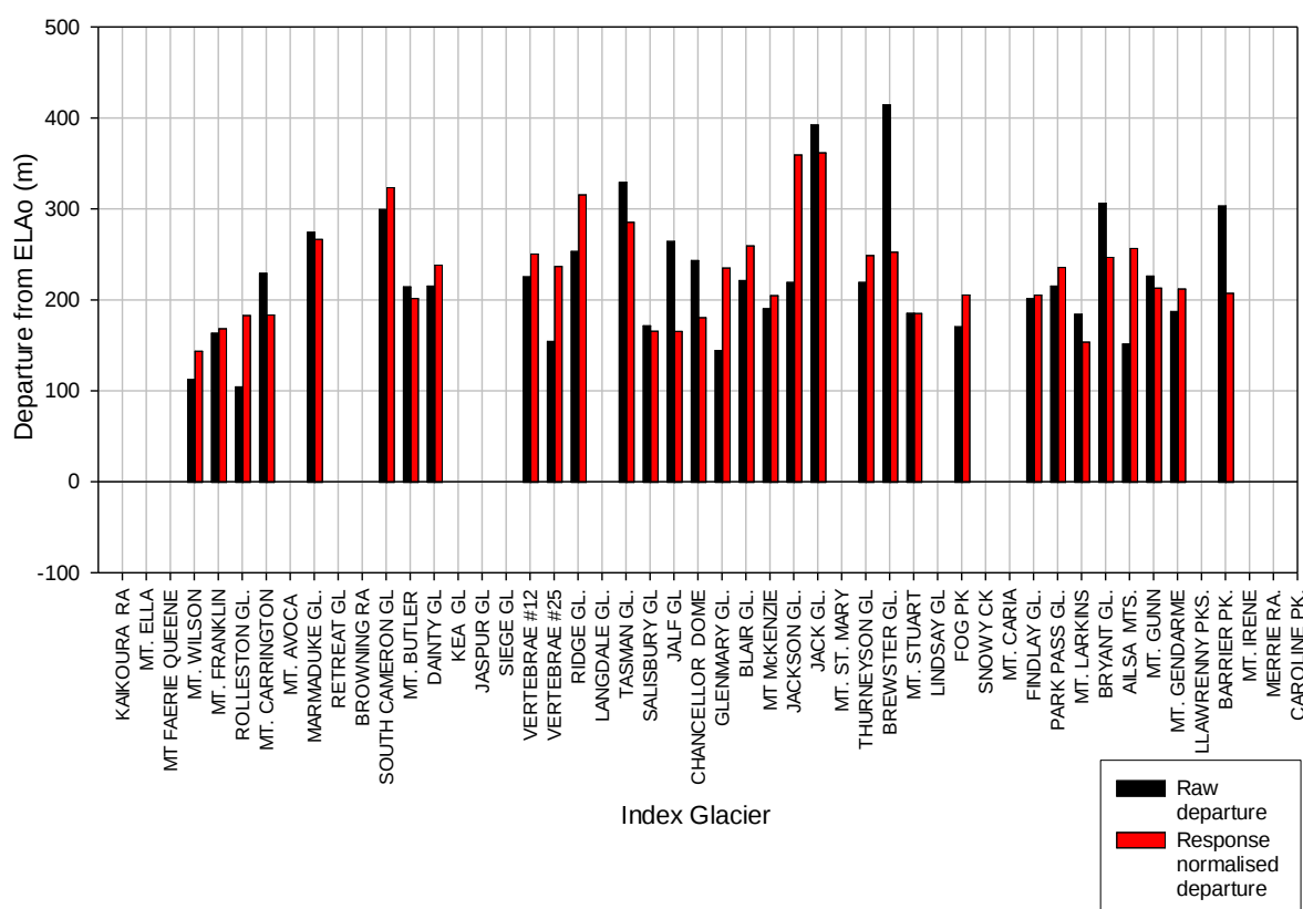
Figure 7: Histogram plot of the 2017/2018 snowline departures (raw and response normalised) for each index glacier from the long-term ELAo. Missing values are due to either the glacier not being visited, used, or the snowline was above the maximum elevation of the glacier.
