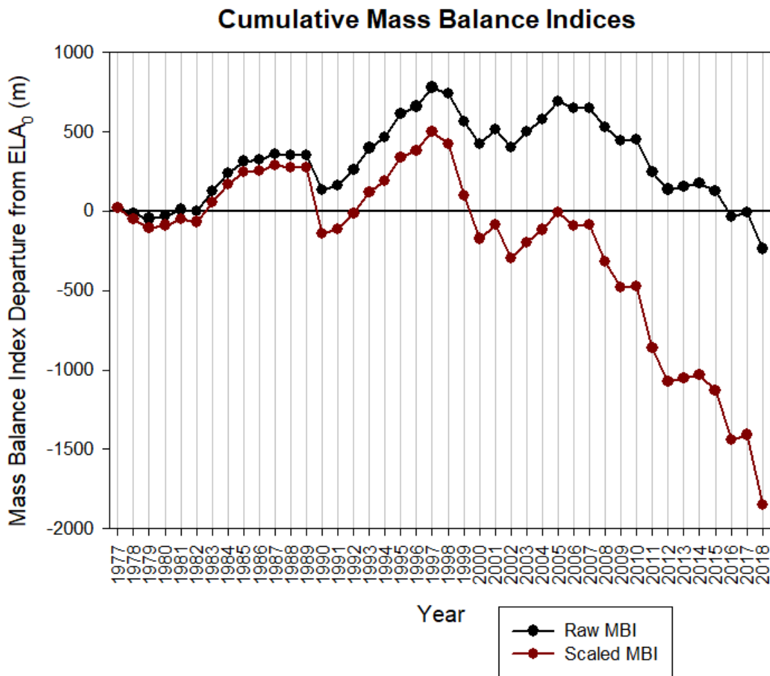
Figure 9: Raw and Scaled Cumulative Mass Balance Indices for the index Glaciers.
