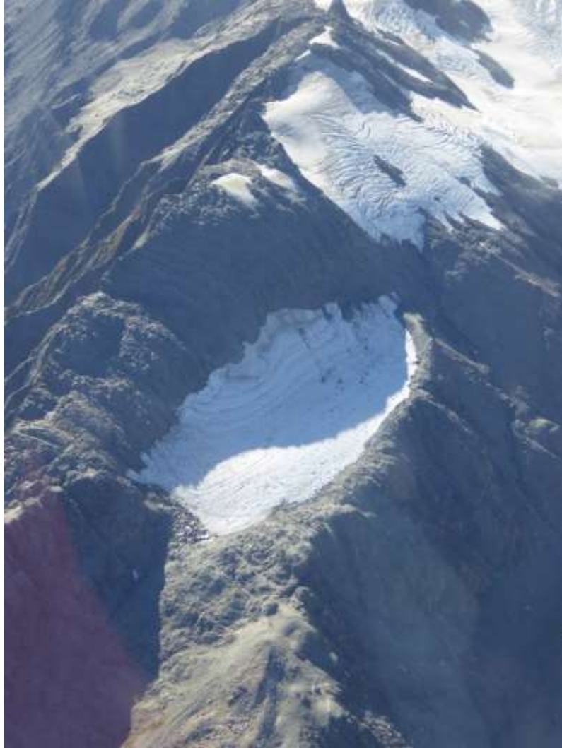
Figure D-23: Chancellor Glacier on 11 March 2018.
