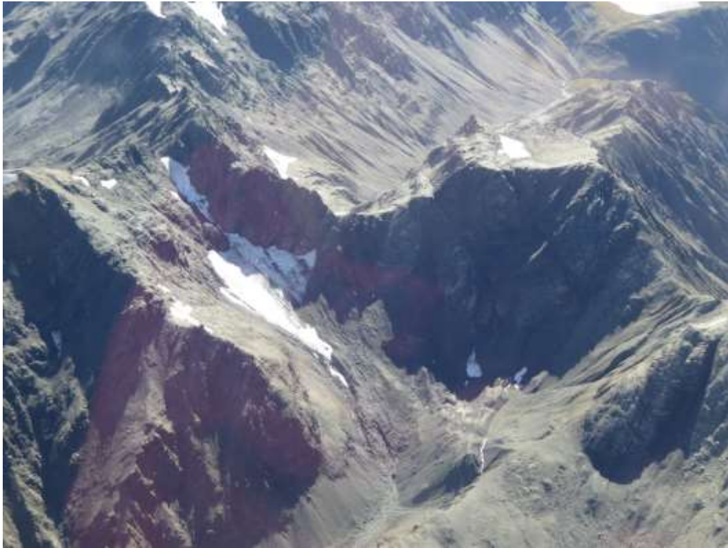
Figure D-7: Retreat Glacier 11 March 2018.
