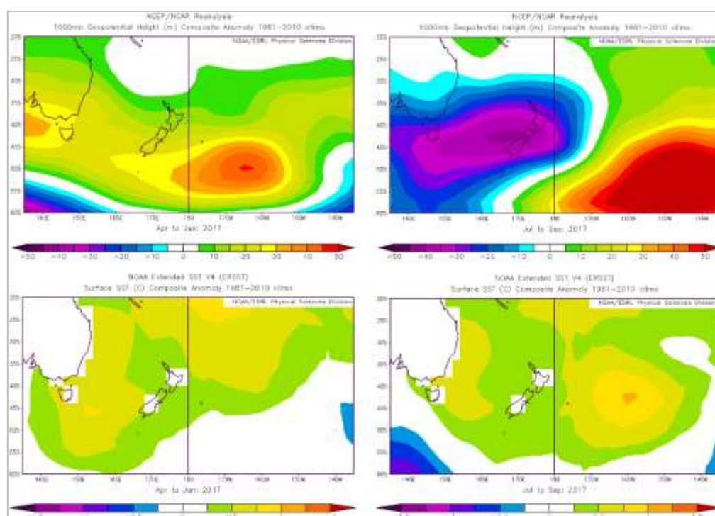
Figure 5: Southwest Pacific anomalies at the 1000hPa geopotential height (top row) April-June 2017 (left) and July-September 2017 (right). Geopotential indicates areas of relatively high or low pressure (green/red shades indicating 'highs', blue/purple shades indicating 'lows'). The bottom row shows the corresponding sea surface temperature (SST) anomalies across the New Zealand sector for the same time period (green/red shades indicating warmth, blue/purple shades indicating cool).
